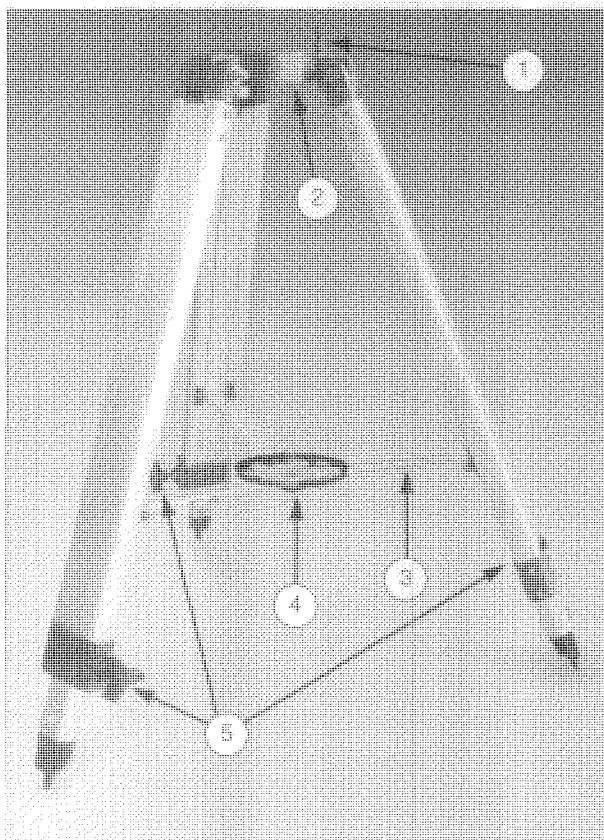
Fig. 2 LXD 500 Tripod. (1) Azimuth Tangent Arm; (2) Tripod Head; (3) Extension Strut; (4) Accessory Tray; (5) Height Adjustment Knob.
