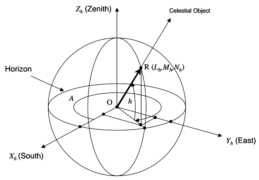
Figure 4-3 Altazimuth Coordinates
