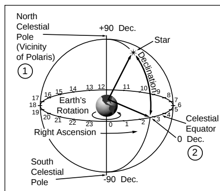
Fig. 25: Celestial Sphere.
