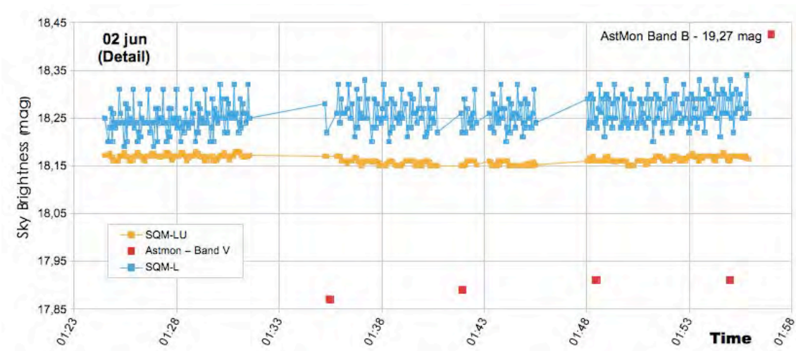
Figure 22: Comparison among corrected measurements acquired with SQM-L units, SQM-LU and AstMon-UCM. SQM-LU measurements are within a narrow range, despite the influence of manipulation.
