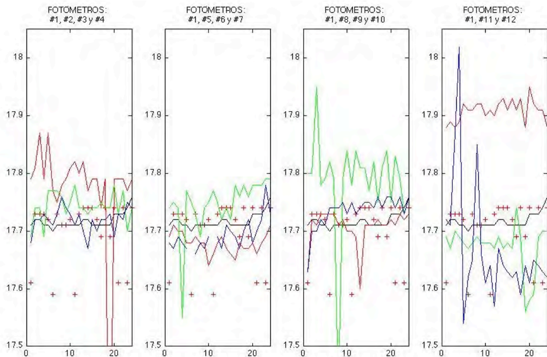
Figure 12: One of the experiences performed thanks to the help of volunteers. A black line always represents SQM SEA #01. Measurements for the rest of units are represented by lines according to their running number: red, green and blue. SQM-LE entries are represented by red crosses, pointing out that the variability range is about 0.10 mag.
