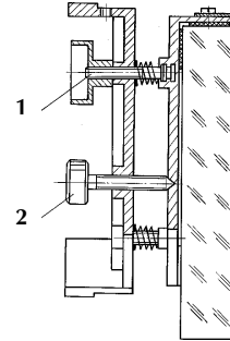
Fig. 3. Primary mirror: 1 - set screw; 2 - adjusting screw
