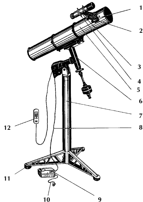
Fig. 1. General view of telescope with metal pier:
