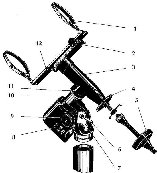
Fig. 5. Equatorial Mounting:
