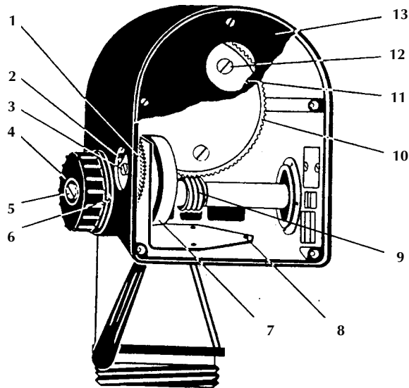
Fig. 10. Watch drive:
