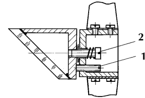
Fig. 4. Diagonal mirror: 1 - adjusting screw; 2 - set screw
