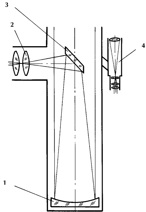
Fig. 7. Optical train of telescope:
