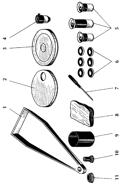
Fig. 9. Tools and accessories:
